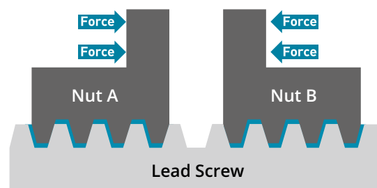
Compression Anti-Backlash Nut
