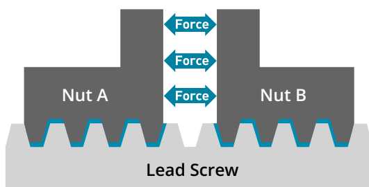
Tension Anti-Backlash Nut
