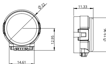
EK 1 Encoder - differential output
