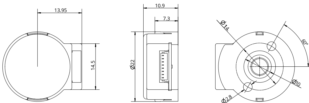
EK 5 Encoder - differential output
