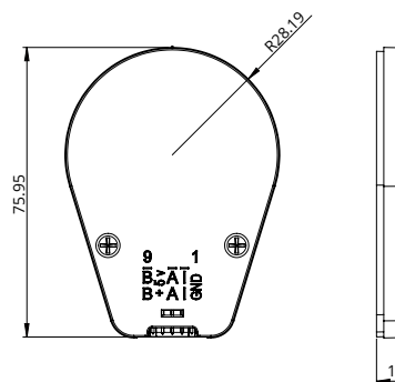
EK 3 Encoder - differential output
