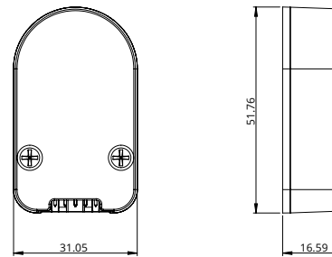
EK 2 Encoder - differential output
