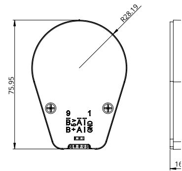
EK 3 Encoder - differential output
